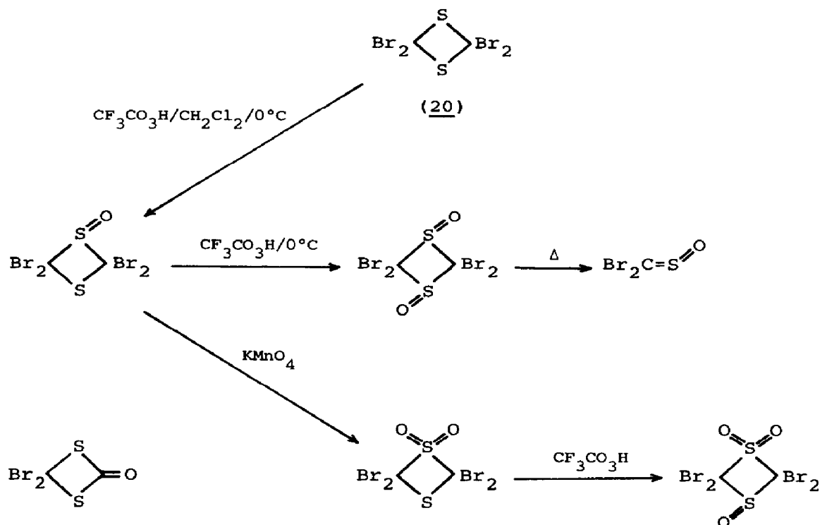
Scheme 5
