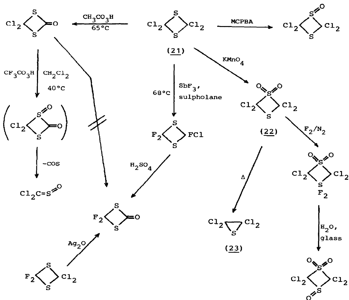
Scheme 6
