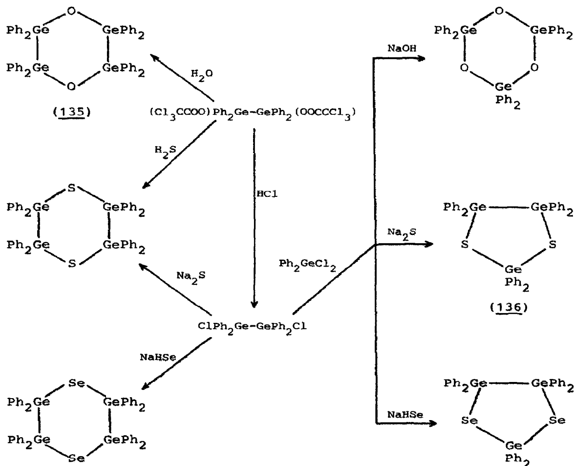
Scheme 22
