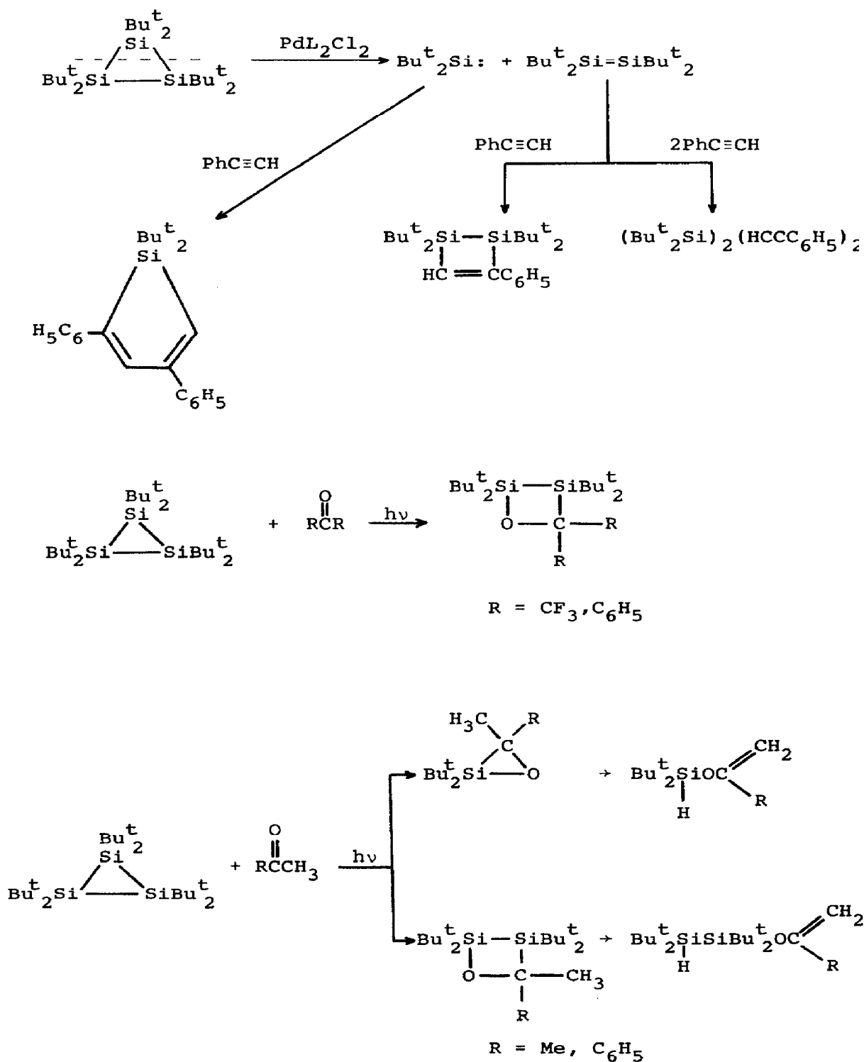
Scheme 8
