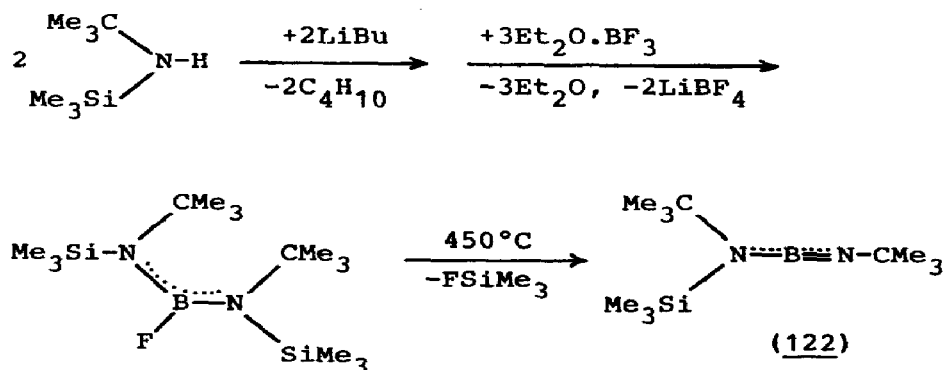
Scheme 19
