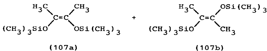
Scheme 18
