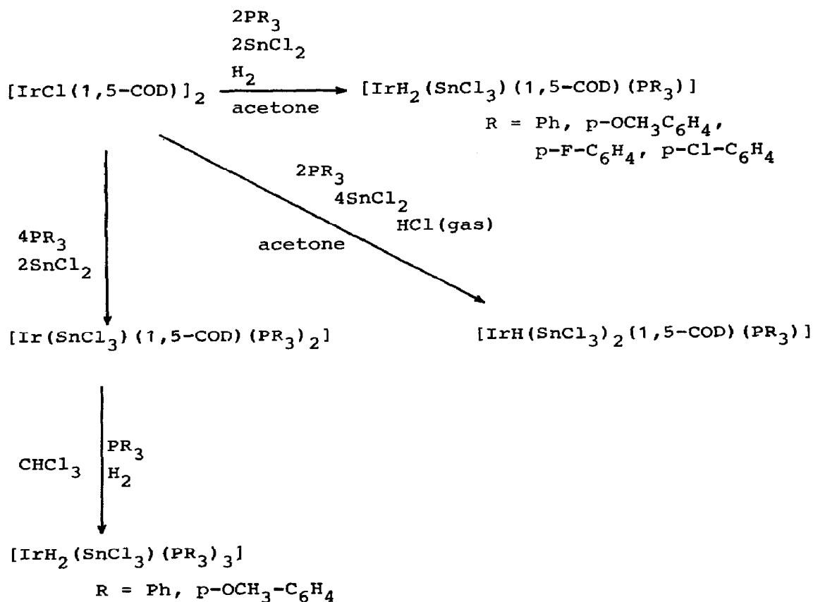
Scheme 26
